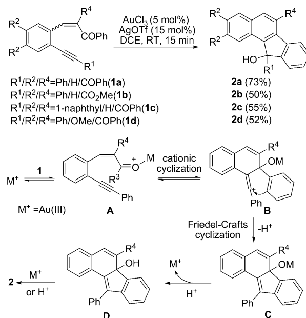
Scheme 1. Gold(III)-catalyzed cationic domino cyclization and the plausible mechanism. DCE = 1,2-dichloroethane, M = gold, Tf = trifluoromethanesulfonyl
