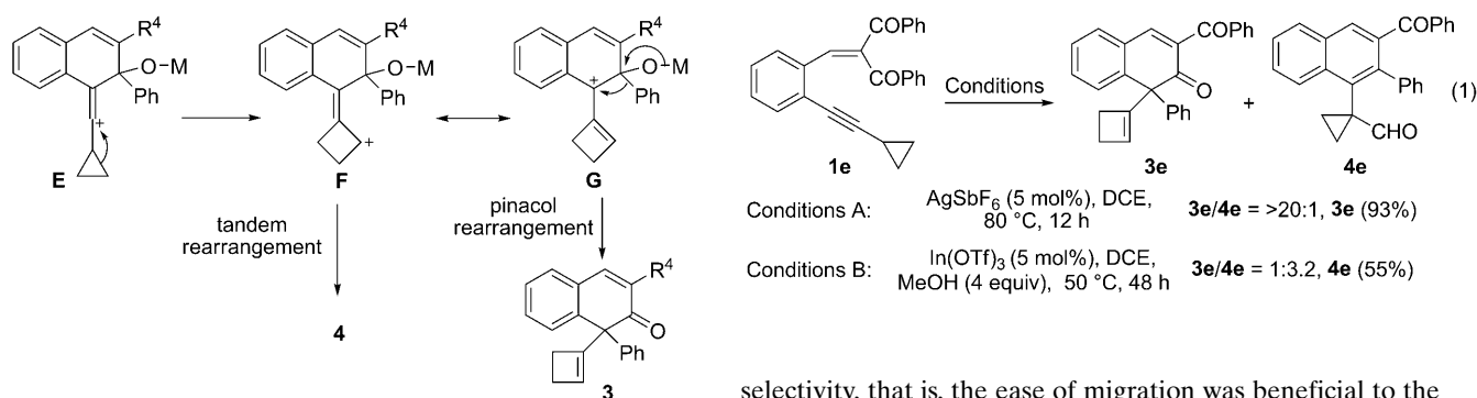
Scheme 2. Projected divergent termination of tandem cationic cyclization/ring expansion reactions of a cyclopropyl substituted substrate.
